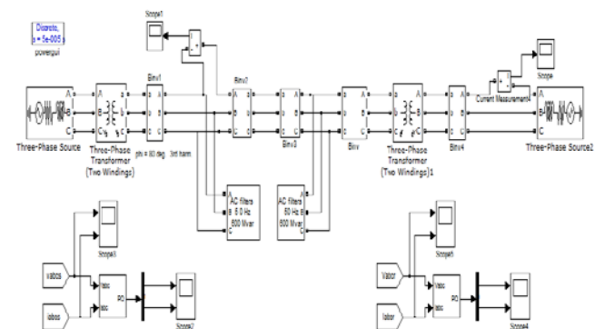
Fig. 5.1 Simulink model using HV AC Transmission
