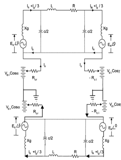
Fig. 3.2: Equivalent Circuit
