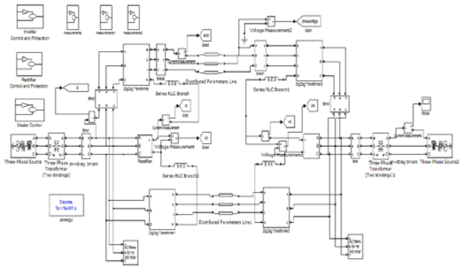
Fig. 5.3: Simulink model using AC-DC Transmission
