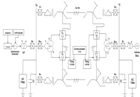
Fig. 3.1: Scheme for composite ac-dc transmission
